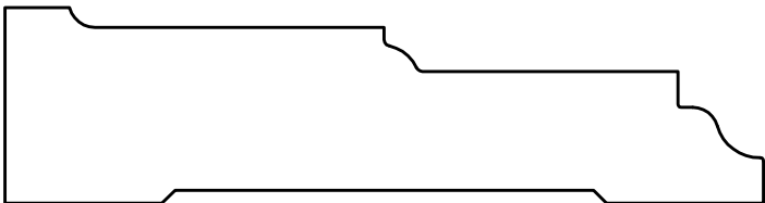
MV1108 - 15/16" x 3 5/8"
