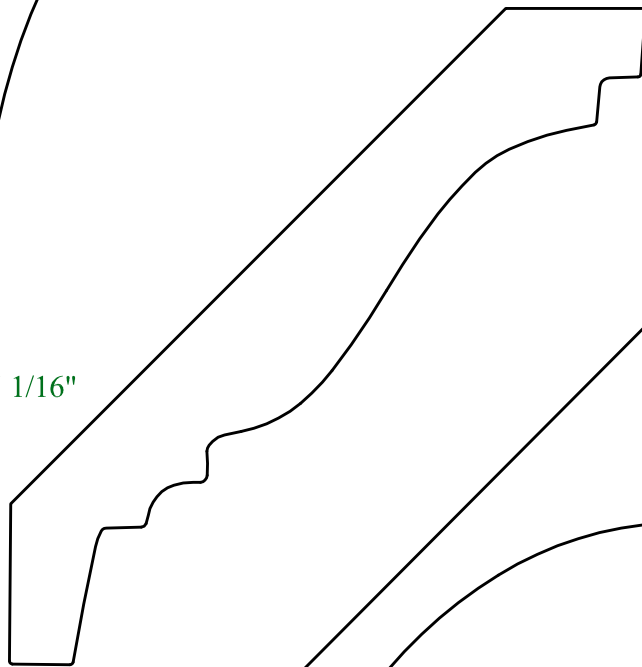
MV378 - 13/16" x 4 3/4"
