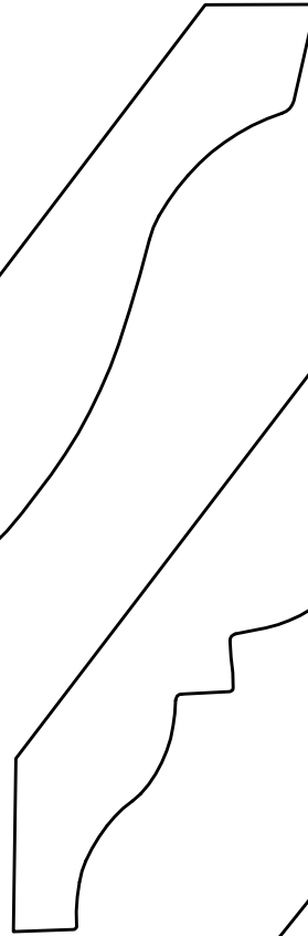
MV351 - 3/4" x 4 1/4"
