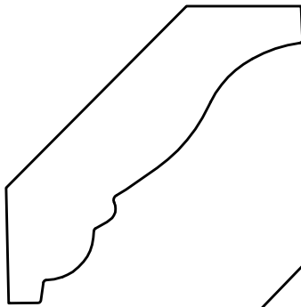
MV330 - 5/8" x 2 7/16"
