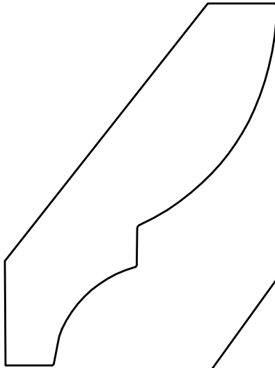
MV340 - 13/16" x 3 3/8"
