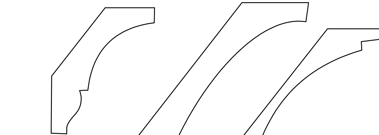
MV367 - 13/16" x 2 3/4"
