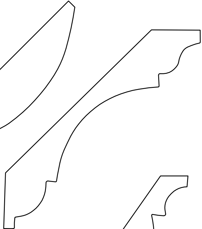
MV336 - 13/16" x 4 7/8"
