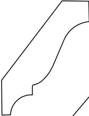
MV302 - 5/8" x 2 5/8"
