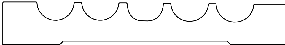
MV167 - 3/4" x 5"
