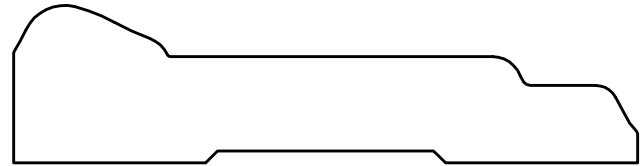
MV1129 - 13/16" x 3 1/4"
