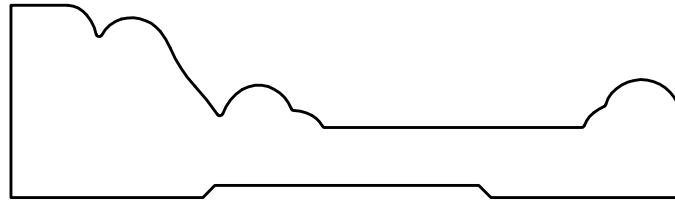
MV1119 - 1" x 3 1/2"
