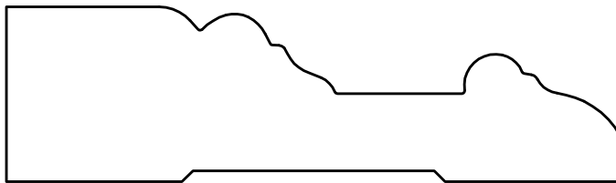
MV1121 - 1" x 3 1/2"
