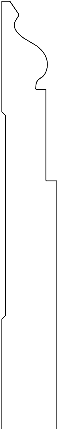
MV290 - 1" x 7 3/4"
