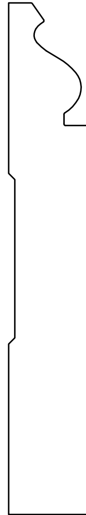
MV296 - 13/16" x 5 1/4"
